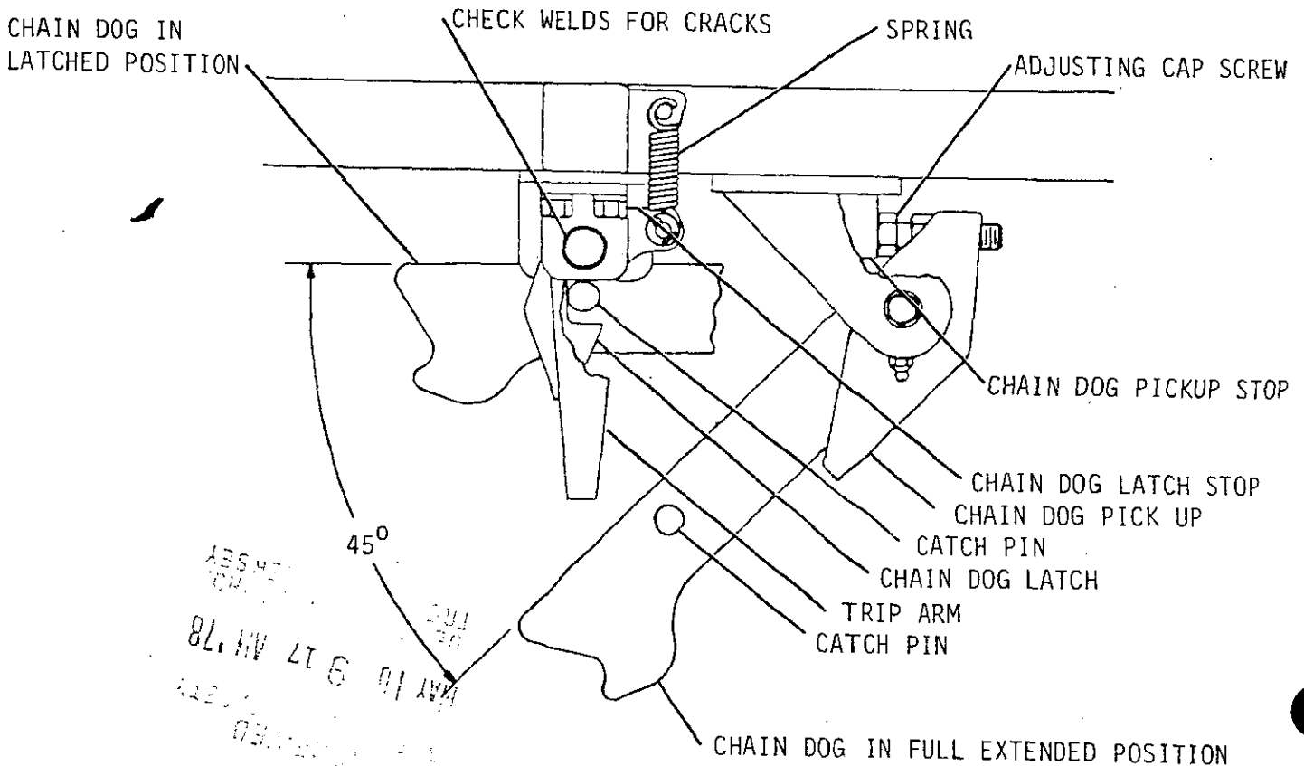
CHAIN DOG ASSEMBLY
